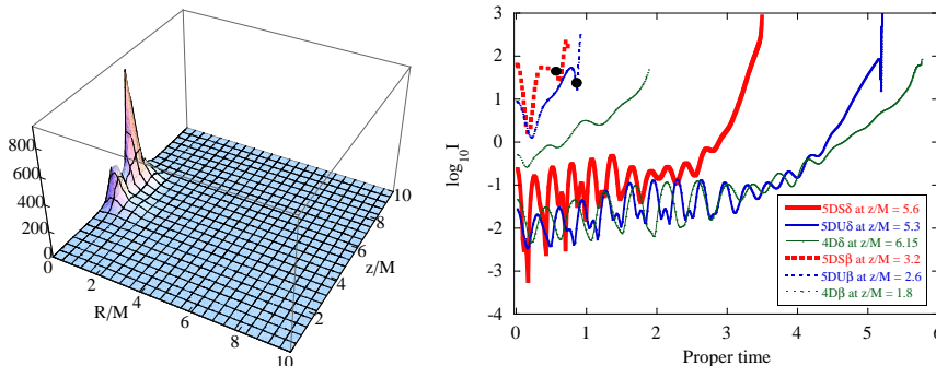
Fig. 3. (Left) Kretschmann invariant \mathcal{I} for model 5DS\delta at t/M = 15.4 . The maximum is O(1000) , and its location is on z -axis, just outside of the matter. (Right) \mathcal{I} at the location of \mathcal{I}_{\max} on the final hypersurface is plotted as a function of proper time at its location. Labels indicate model-names in Table 1. The time of AH formation ( t=0.6 for model 5DS\beta , t=0.9 for 5DU\beta ) is shown by a dot.
