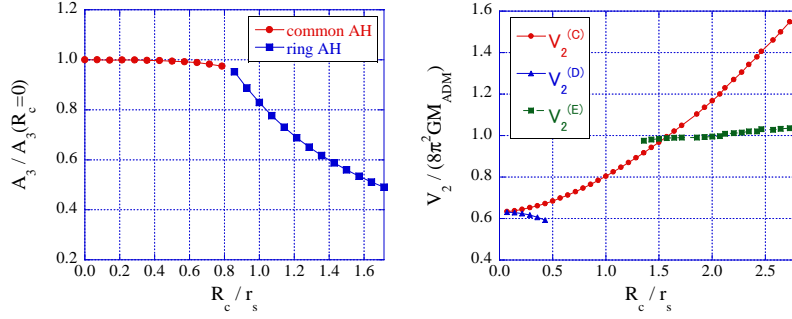
Fig. 5. (Left) The area of the apparent horizon A_3 . Plots are normalized by the area of spherical case ( R_c = 0 ). We see both horizons' area are smoothly connected at R_c/r_s = 0.78 , and both monotonically decrease with R_c/r_s . (Right) The ratio of the hyper-hoops V_2 to the mass M_{ADM} are shown for the sequence of Fig.1. The ratio less than unity indicates that the validity of the hyper-hoop conjecture.
