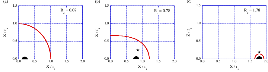
Fig. 4. Matter distributions (shaded) and the location of the apparent horizon (line) for toroidal matter configurations. The asterisk indicates the location of the maximum Kretschmann invariant, \mathcal{I}_{max} .
