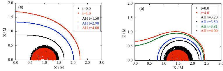
Fig. 6. Snapshots of evolutions of ring-shaped matter: for the initial data of (a) R_c/M = 1.00 and (b) 1.50, both with no AHs on the initial hypersurface. The matter distribution at t = 0.00 and t = 4.00 , and the location of AHs are plotted on X - Z coordinates. We see that AH topology switches from toroidal to spherical in (b).
