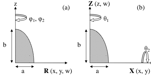
Fig. 1. We evolve five-dimensional (a) axisymmetric [SO(3)] or (b) double-axisymmetric [ U(1) \times U(1) ], asymptotically flat space-time using the Cartesian grid. The initial matter configuration is expressed with parameters a and b .
