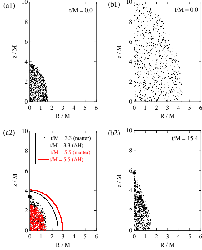
Fig. 2. Snapshots of 5D axisymmetric evolution with the initial matter distribution of b/M = 4 [Fig.(a1) and (a2); model 5DS \beta in Table 1] and 10 [Fig.(b1) and (b2); model 5DS \delta ]. We see the apparent horizon (AH) is formed at the coordinate time t/M = 3.3 for the former model and the area of AH increases, while AH is not observed for the latter model up to the time t/M = 15.4 when our code stops due to the large curvature. The big circle indicates the location of the maximum Kretschmann invariant \mathcal{I}_{\max} at the final time at each evolution. Number of particles are reduced to 1/10 for figures.
