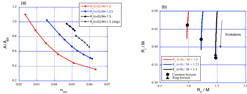
Fig. 7. (a) Area of AH is plotted as a function of minimum lapse function \alpha_{\min} for three cases. We see AH increases monotonically, and jumps when the topology changes. (b) The ring matter configuration (R_c, R_r) with marks when the horizon forms during its evolution.
